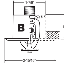
Standard Recessed Escutcheon (3/4" Adjustment)
