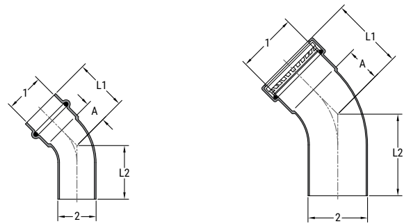
SP649 CU P X MS STREET 45 ELL
