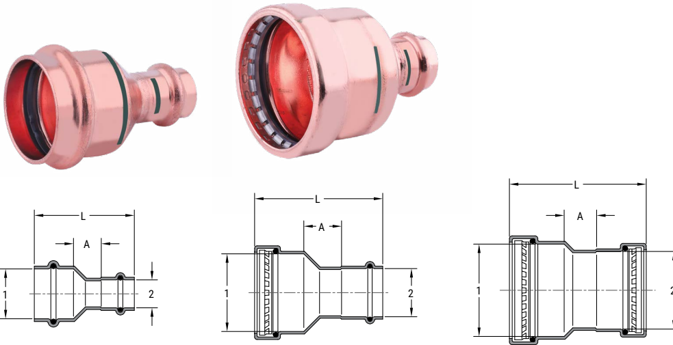
SP604R CU P X P RED COUPLING
