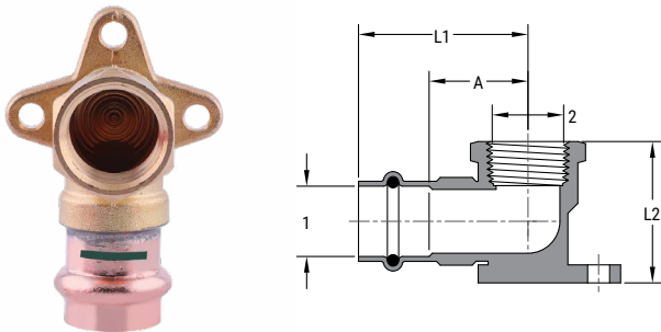
SP698DE P X FPT DROP EAR 90
