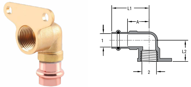
SP698HE P X FPT HI EAR 90
