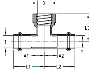
SP628 CU P X P X FT ADPT TEE
