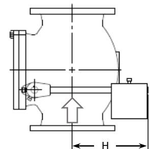
VERTICAL INSTALLATION
