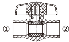
COMPACT BALL VALVE W/EPDM O-RING (SOC × SOC)
