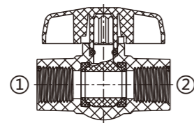
COMPACT BALL VALVE W/EPDM O-RING (FIPT × FIPT)
