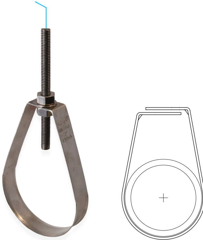
Fig. 69SSG: Dimensions (in) • Loads (lbs) • Rod Size (in)
