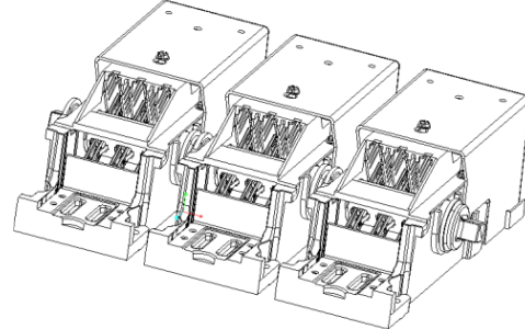
Figure 9. : Line Shield THSHLD5A & THSHLD6A for Safety Switch
