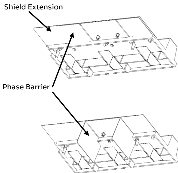
Figure 4. : Arc Shield THSHLD4 for Safety Switch
