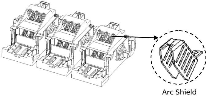
Figure 7. : Arc Shield Assembly THSHLD5A & THSHLD6A for Safety Switch
